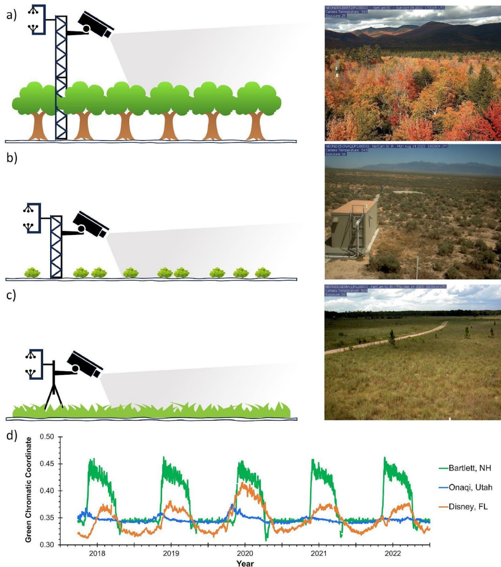
Figure 1. Examples of PhenoCam installations in three ecosystem types: a) a 30+ m tower above forest canopy (Bartlett, NH), b) a 10+ m tower in desert shrubland (Onaqui, UT), and c) a 3+ m tripod in temperate grassland (Disney, FL). d) Green chromatic coordinate ( G_{CC} ) data during a five-year period illustrate the differences in timing, magnitude, and regularity of phenology across ecosystem types (adapted from Richardson, 2023b).
