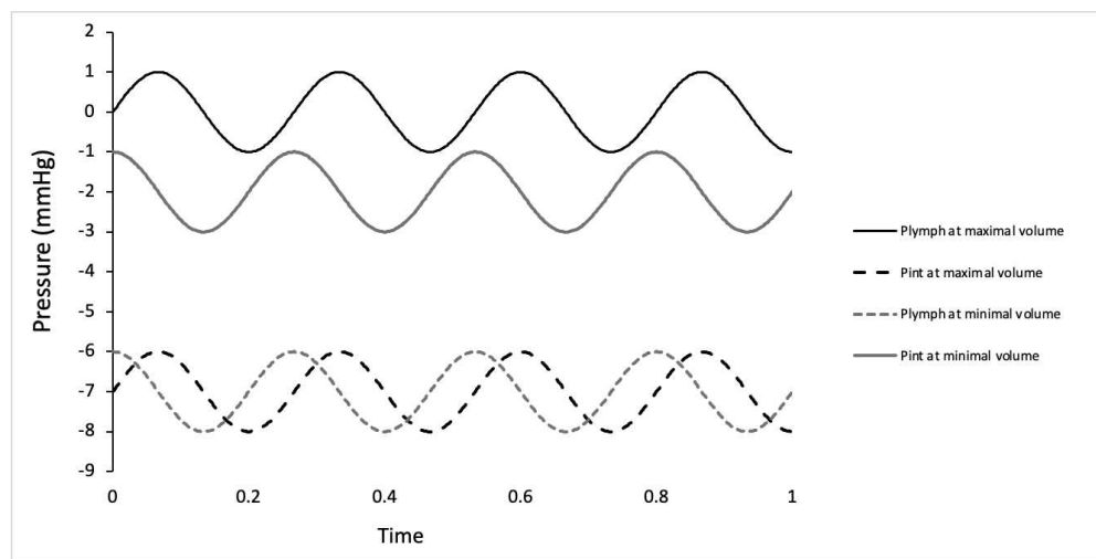
Figure S1: Plot of pressure versus time demonstrating the sinusoidal relationships for the hydrostatic pressure in the interstitial space (Pint, Equation S4) and hydrostatic pressure in the lymph space (Plymph, Equation S6).
