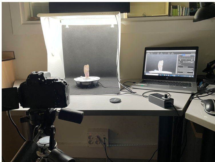
Fig. 3: Set up with the camera at a front angle, connected to the Helicon Remote .
