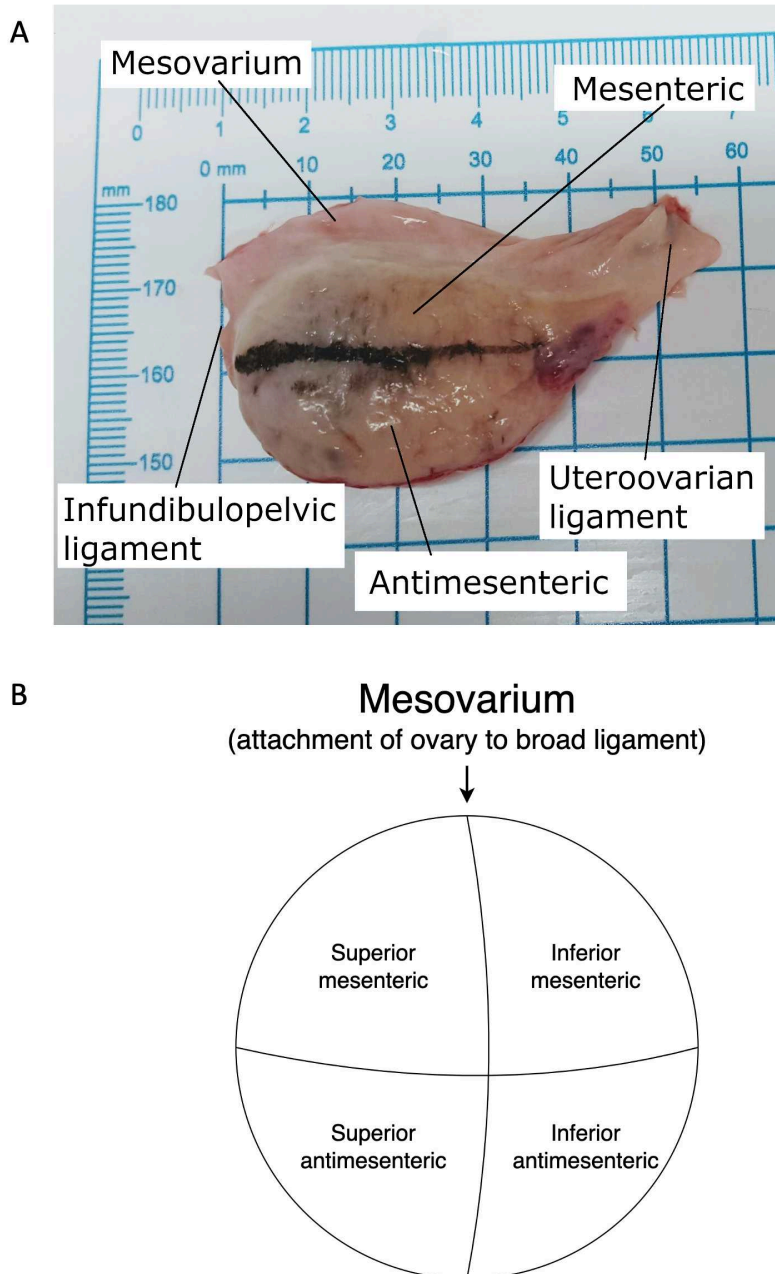
Figure 1. Use of fixed anatomic structures in the ovary. There is laxity in the structures supporting the position of the ovary which results in both intra- and inter-individual variations in the organ's orientation within the pelvis. In order to standardize collection and maintain orientation of tissue sections, a model proposed at a NICHD-sponsored workshop that used fixed anatomic structures to create a regional map of the ovary, was applied. Here the black line was drawn on the inferior half of the ovary when it is divided by its attachment to the mesovarium. The line delineates the mesenteric and antimesenteric portions of the inferior aspect of the right ovary.
