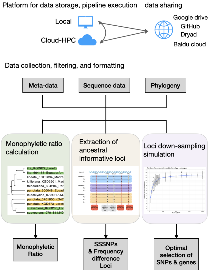
Figure 1. Overview of the data management and the structure of NucBarcoder. The data storage and pipeline execution are performed on both a local computer and a High-Performance Computing system via cloud service. The original data from public and private providers is deposited and downloaded from Google Drive, Dryad, and Baidu cloud. The data underwent format tidying up and filtering locally and was then uploaded to HPC for intensive processing and analytical tasks. The Nucbarcoder pipeline comprises three main parts: Monophyletic ratio calculation, Extraction of ancestry informative loci, and loci down-sampling simulation (sub-sampling of the data).
