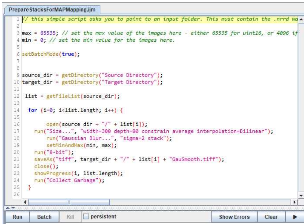
The ImageJ macro "PrepareStacksforMAPMapping.ijm"
