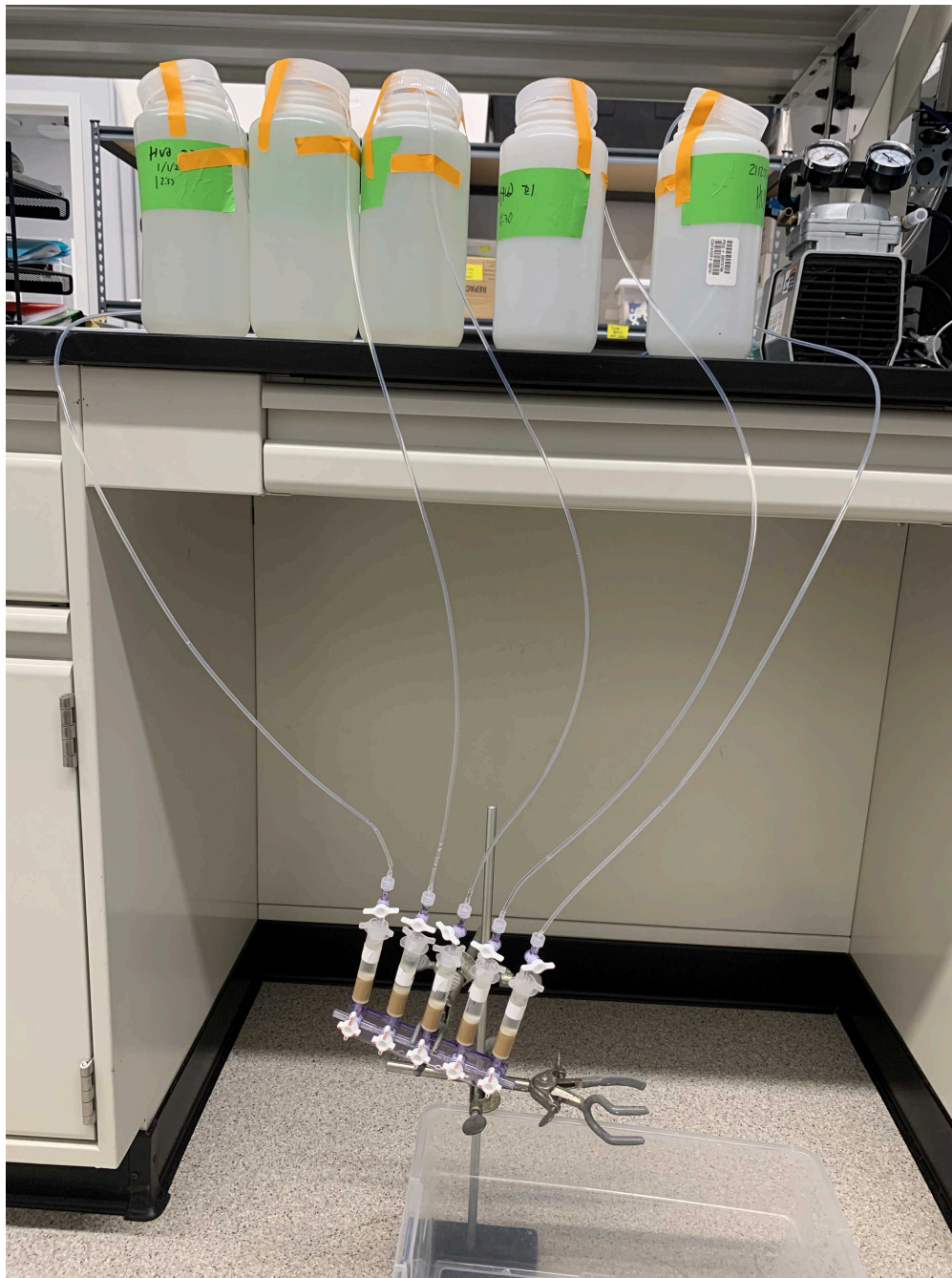
Image of SPE apparatus for 5 samples.
