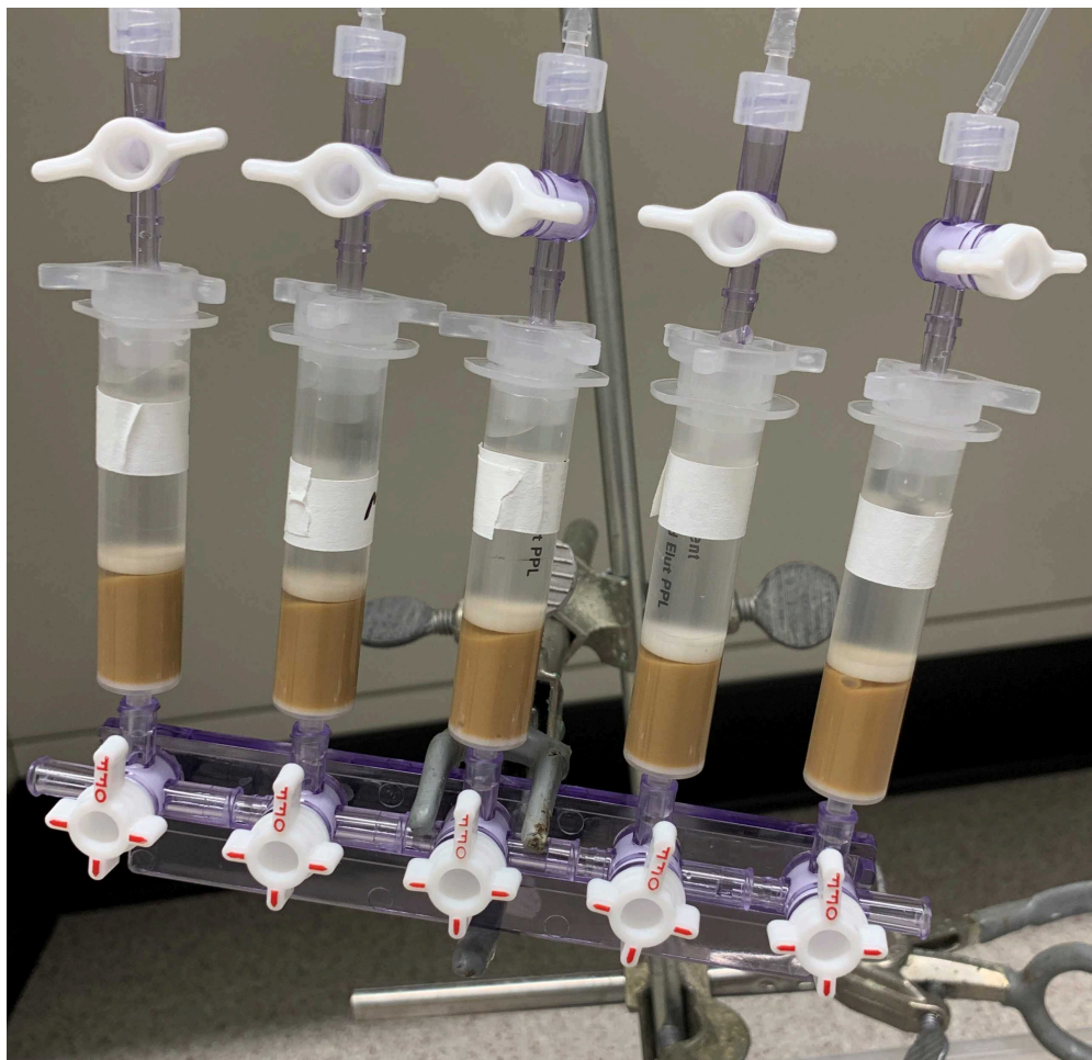
Image of full manifold.
