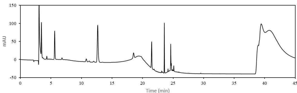
Chromatogram of dissolved organic matter sample
