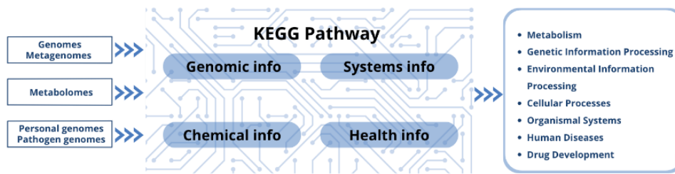
Fig 2: KEGG flowchart
