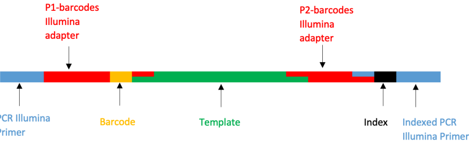
Final ddRAD library construction
