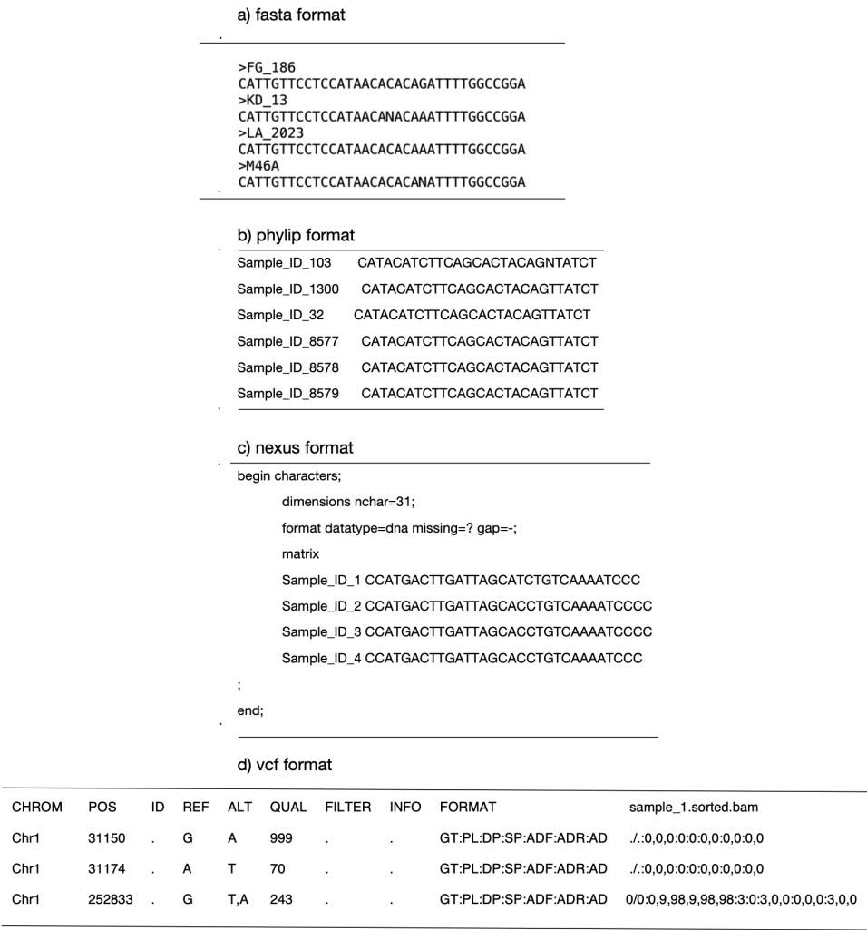
Figure 3.2. Examples of aligned sequences in a) fasta, b) phylip, and c) nex formats, and SNP matrix in d) vcf format.
