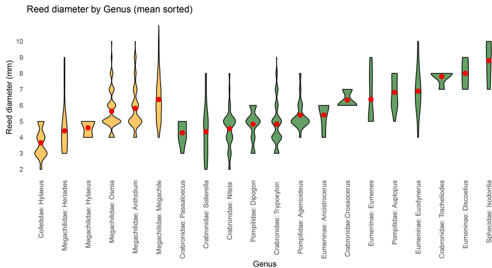
Figure 1: Cavity size preferences of different Hymenoptera genera. Most cavity-nesting species utilise reed stems with an inner diameter between 3 and 8 mm. However, providing a uniform distribution of diameters ranging from 2 to 12 mm is recommended to avoid excluding smaller or larger-bodied species. Bees are indicated in orange, wasps in dark green, red dots represent the mean, and the violin plot illustrates the distribution. Data are based on surveys conducted by the authors in East-Central Europe.
